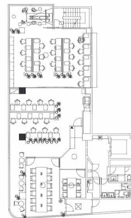
3RD FLOOR
